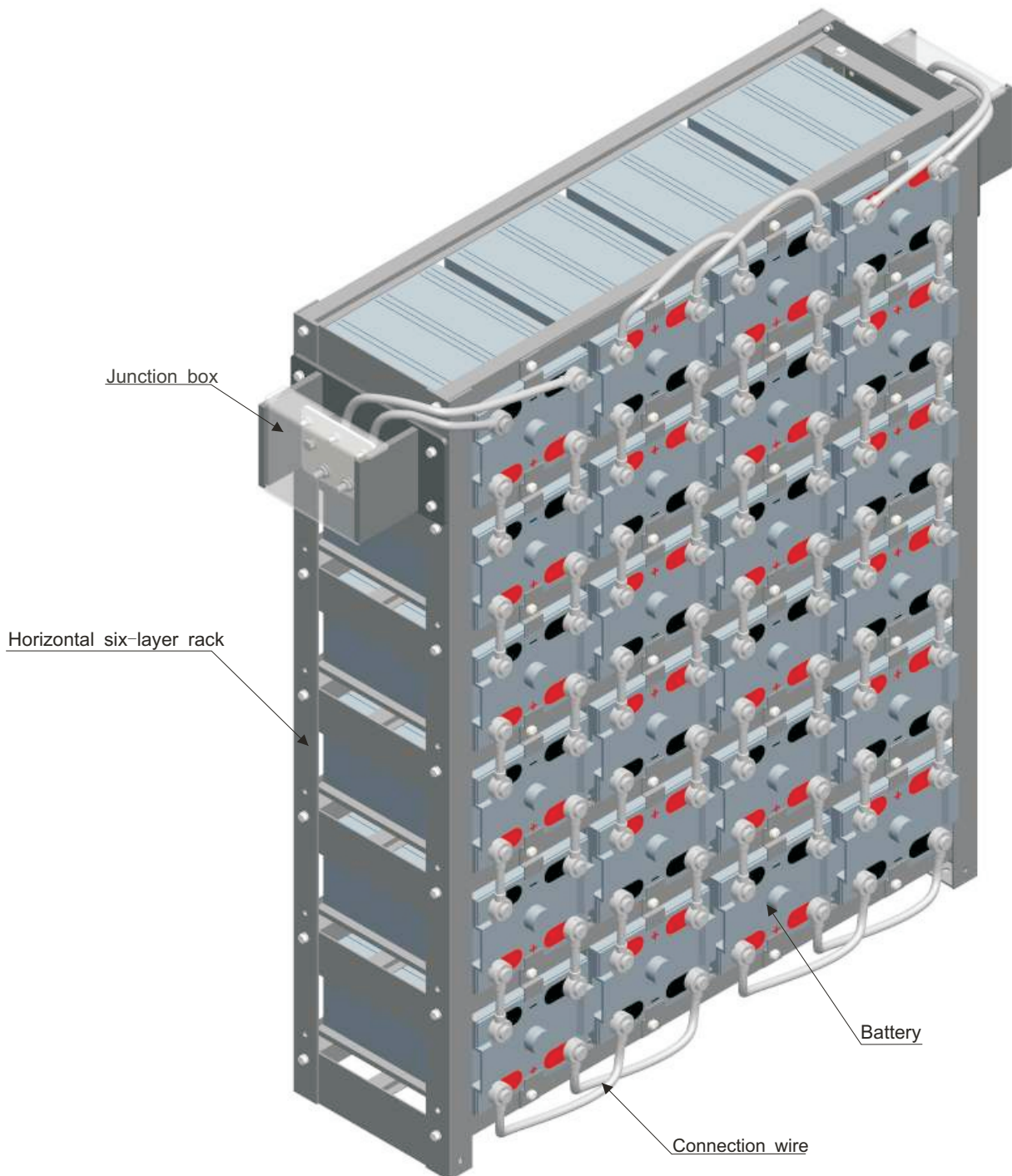
2V horizontal six-layer folded rack with 24pcs batteries
